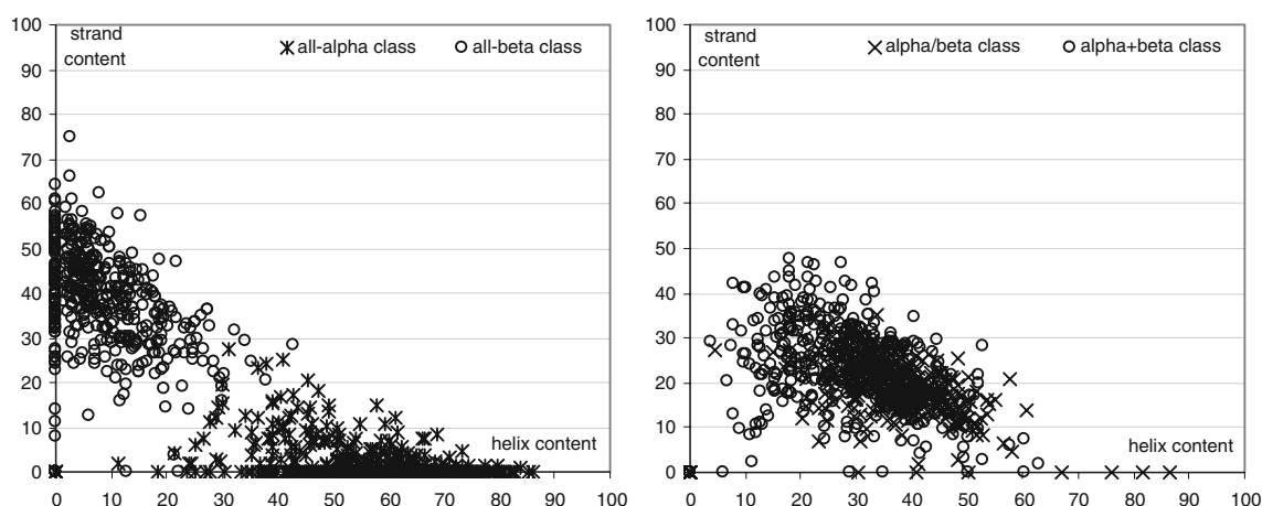
Fig. 4 Scatter plot of helix content (X-axis) against strand content (Y-axis) based on DSSP-assigned secondary structure for proteins in the 25PDB dataset. The left panel shows the plot for the all- \alpha and all- \beta classes, the right panel shows the plots for the \alpha/\beta and \alpha + \beta classes
