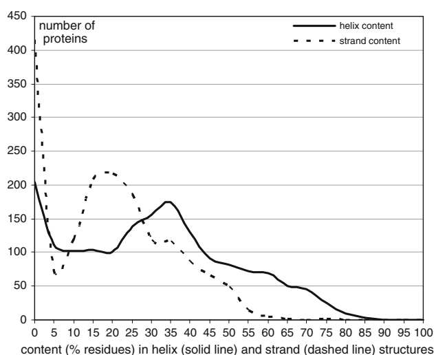
Fig. 3 Distribution of the helix (solid line) and strand (dashed line) content based on Dictionary of Secondary Structure of Proteins (DSSP)-assigned secondary structure for proteins in the 25PDB dataset
